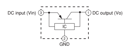
IC3, 11: PQ033ES3MXP Low power loss regulator
