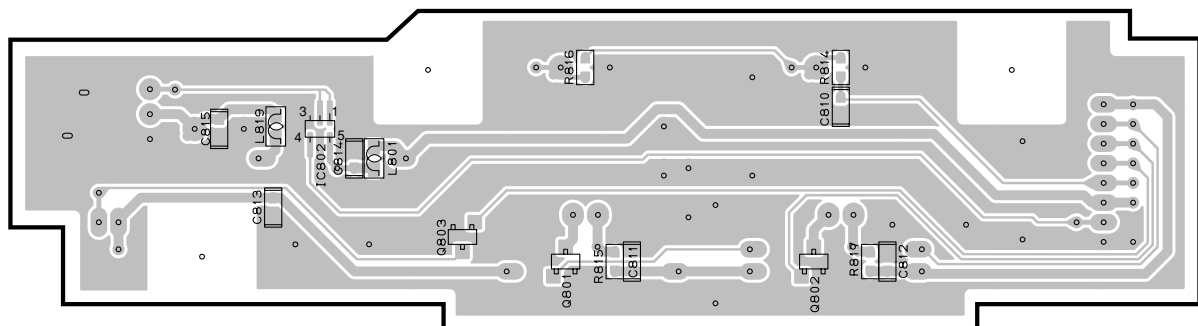
DIGITAL (3) P.C.B. (Side B)
