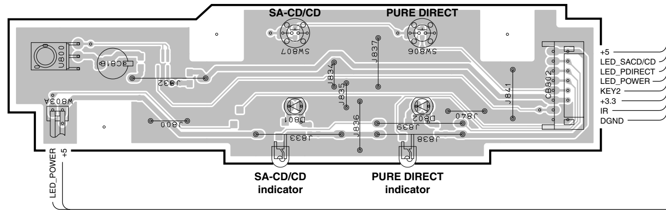
DIGITAL (3) P.C.B. (Side A)
