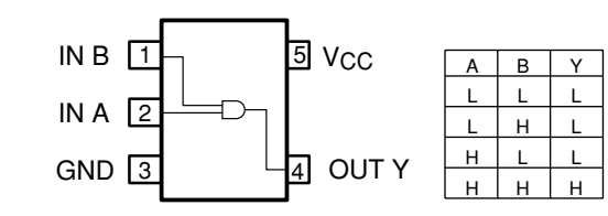
IC802: TC7SH08F 2-input AND gate
